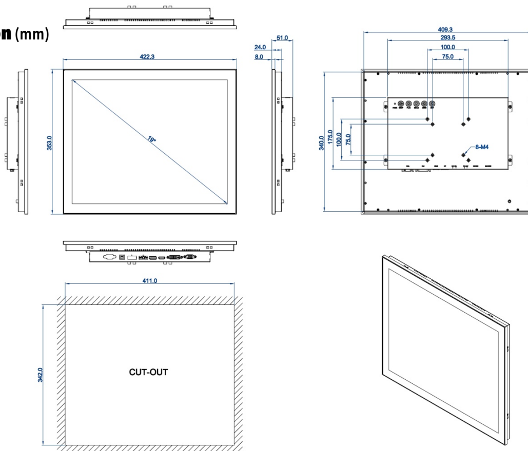
DIMENSIONAL DRAWING:TM-PCA190
