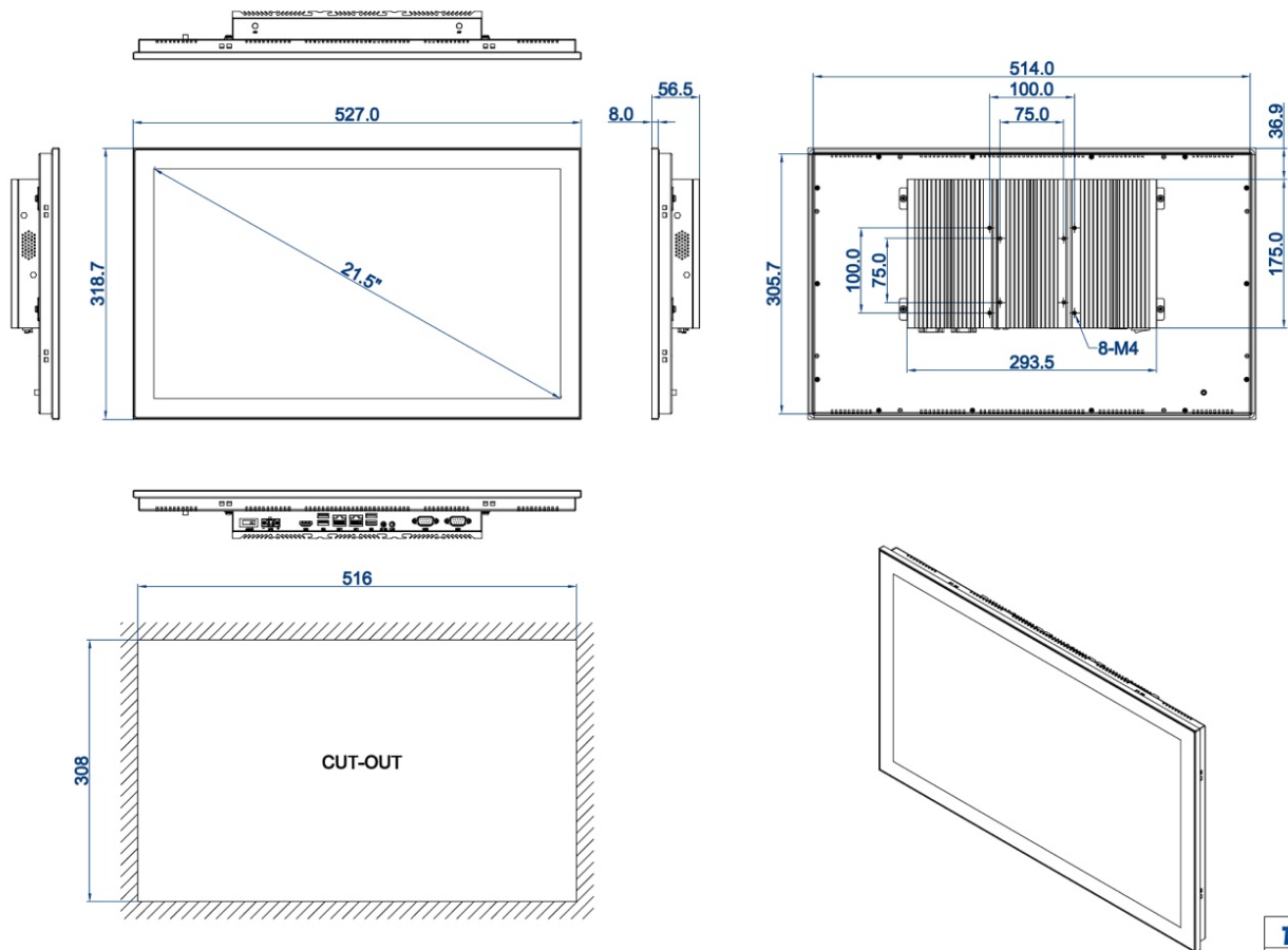
DIMENSIONAL DRAWING:TPC-DCM215
