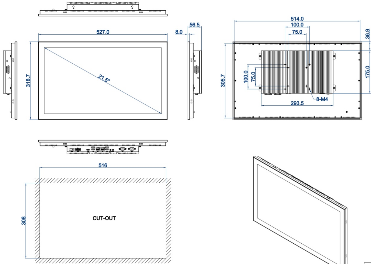
DIMENSIONAL DRAWING:TPC-DCM215
