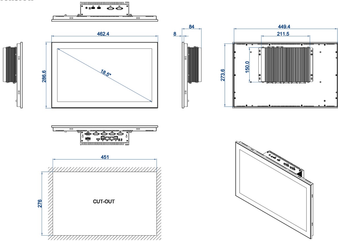
DIMENSIONAL DRAWING:TPC-PC185
