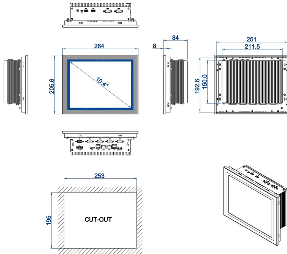
DIMENSIONAL DRAWING:TPC-PR104
